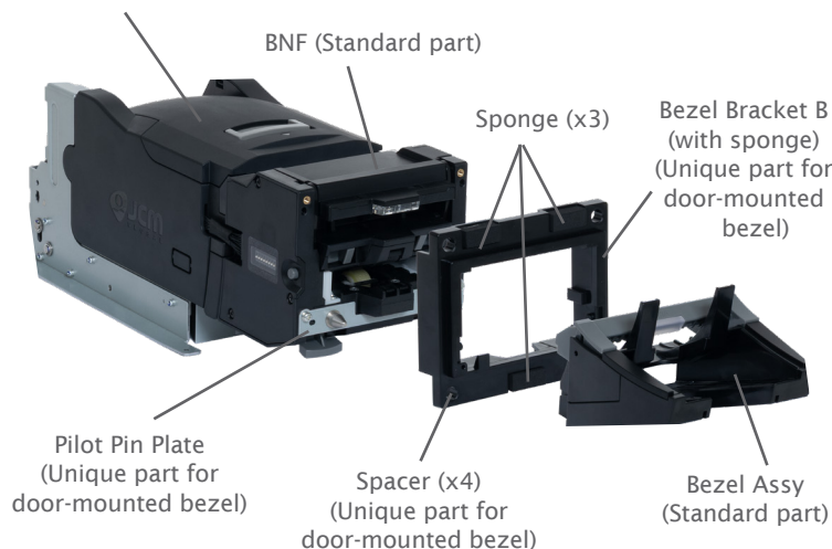
UBA Pro Head (Standard part)
