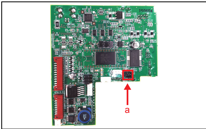
Figure 1 UBA®-10 3.3V CPU with DF3 Motor Connector (P/N 241164)
