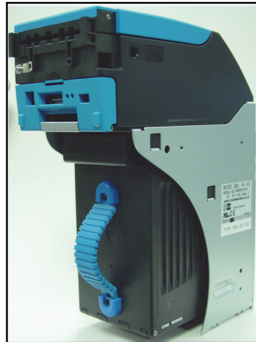
Figure 2: UBA-10 Banknote Acceptor Unit
