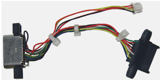
Figure 1 Adapter Harness, iVIZION® to UBA Connector (P/N 40i-000001R)
