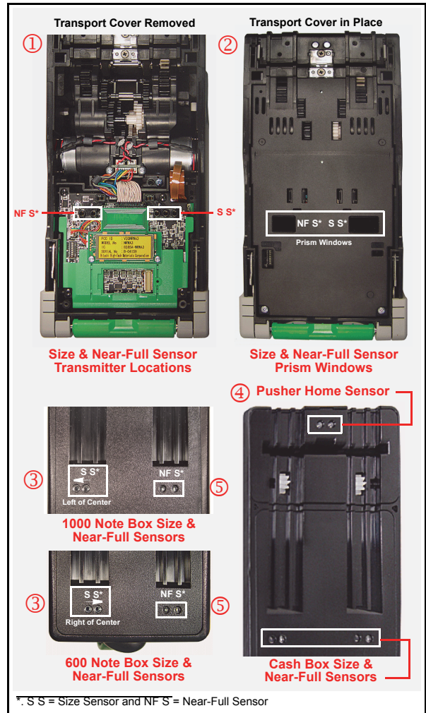
iVIZION Validator & Cash Box Sensor Locations
