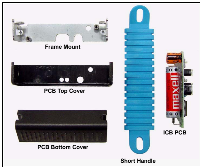
ICB Retrofit Kit Components
