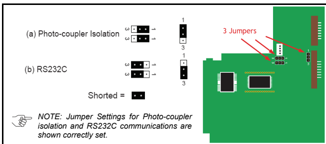
UBA CPU Board Jumper Locations
